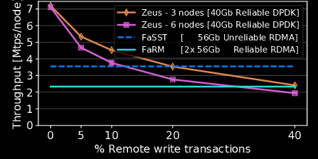
Figure 9. TATP while varying remote write transactions.
