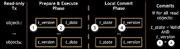
Figure 6. Zeus' consistent read-only transactions on readers.
