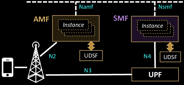
Figure 1: Simplified 5G core network overview (we omit many more control plane elements for clarity).
