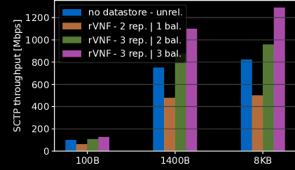
(b) SCTP performance when varying the traffic size [Rack].
