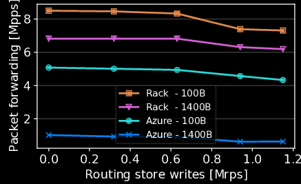
Figure 10: LB micro benchmark: Aggregate packet forwarding rate over 3 LBs as a function of a number of routing KVS writes.
