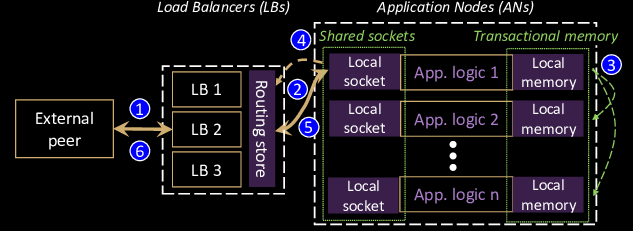
Figure 3: rVNF software architecture. An LB is collocated with an AN on the same physical server.
