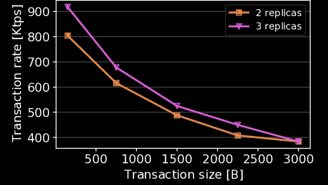
Figure 11: Transaction micro benchmark: Maximum rate for two- and three-way replication and different transaction sizes. [Rack]
