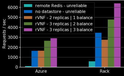
(a) Performance of service requests (per core) for different SGW configurations.
