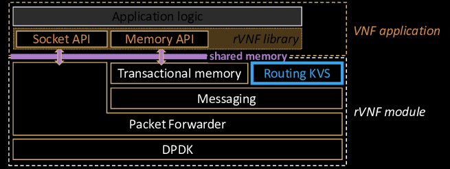
Figure 7: rVNF system architecture. If routing KVS is present, rVNF module acts as an LB. Otherwise, it connects to another node to access a LB.
