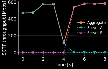
Figure 9: SCTP failover performance. The failure of the primary instance happens at 3s. [Rack]
