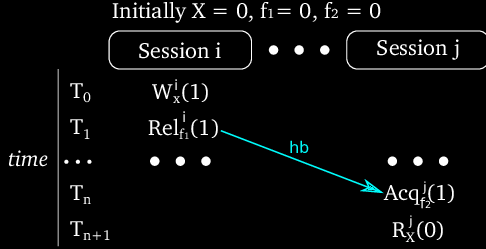
Figure 4. Proof sketch assumed violation. The RC violation is that Session A reads X = init , instead of X = 1 .
