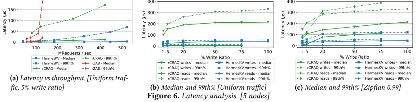
Figure 6. Latency analysis. [5 nodes]
