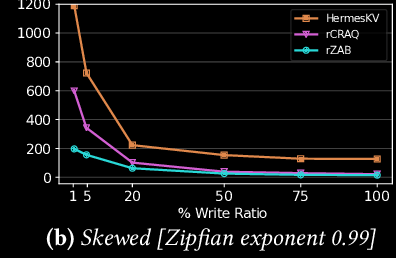
Figure 5. Throughput for 1% to 100% write ratio. [5 nodes]
