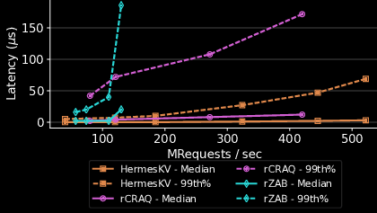
(a) Latency vs throughput. [Uniform traffic, 5% write ratio]
