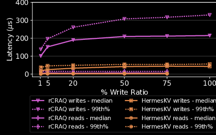
(b) Median and 99th [Uniform traffic]
