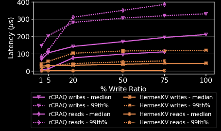
(c) Median and 99th [Zipfian 0.99]
