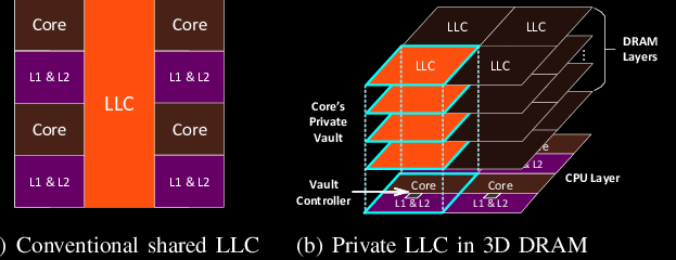
Figure 1. Conventional shared LLC and NG-LLC in a 4-core CPUs. Figure from [2].
